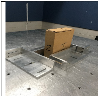
Block 12 Face 6 Test Set up
